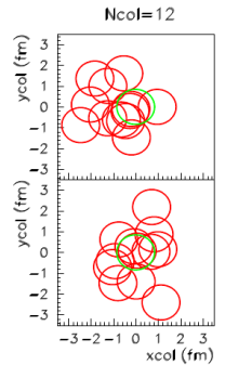
p+Pb 5.02 TeV, b=0
