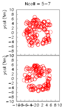
Pb+Pb 2.76 TeV, b=0
