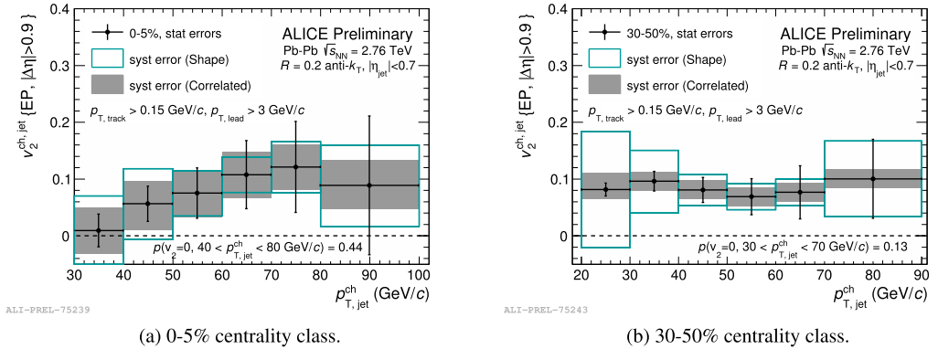
Fig. 3. Charged jet v_2 in Pb–Pb collisions at \sqrt{s_{NN}} = 2.76 TeV at mid-rapidity. Jets are required to have a leading hadron with p_T > 3 GeV/c.
